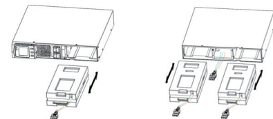
Easy for maintenance, hot-swappable battery
