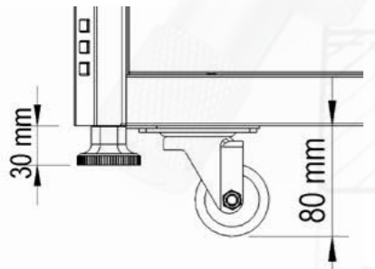
Wheel and Levelling feet
