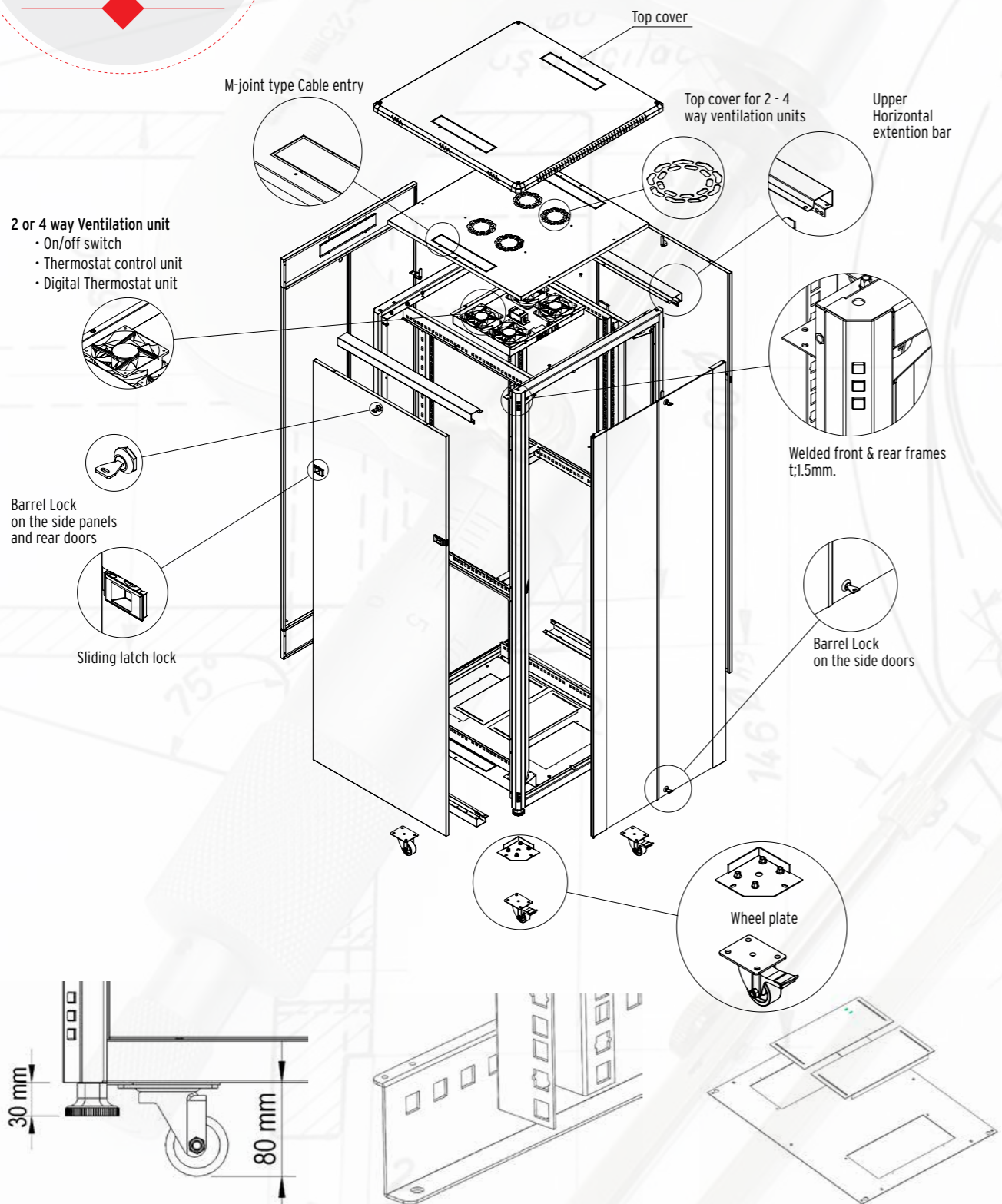
Wheel and Levelling feet
