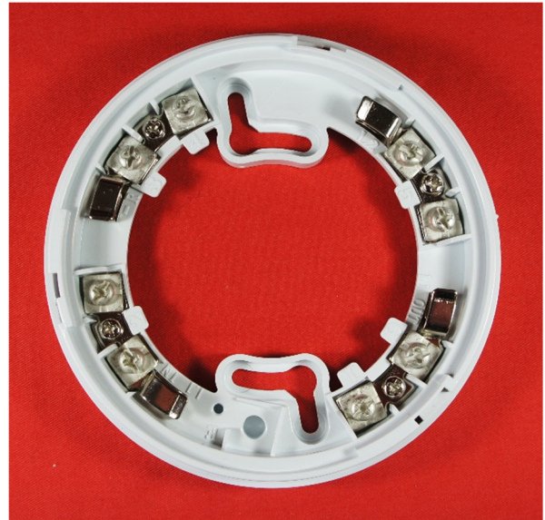
CN304A low profile 102 mm 8-terminal base
