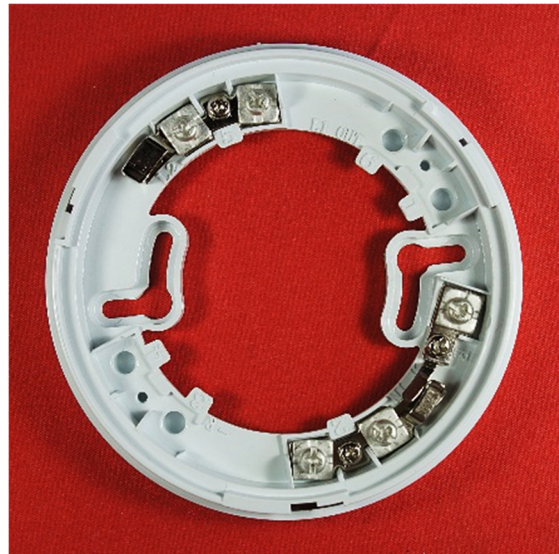
CN3021 / CN3023 low profile 102 mm 5-terminal base
