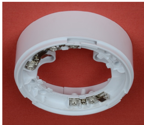
481-002 high profile 102 mm 5-terminal base
